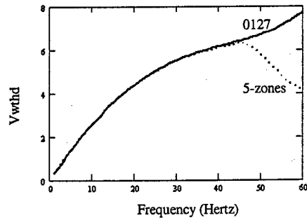
Fig. 29. Analytical results of V_{WTHD} vs. frequency for CSVPWM and Five-Zone hybrid PWM
