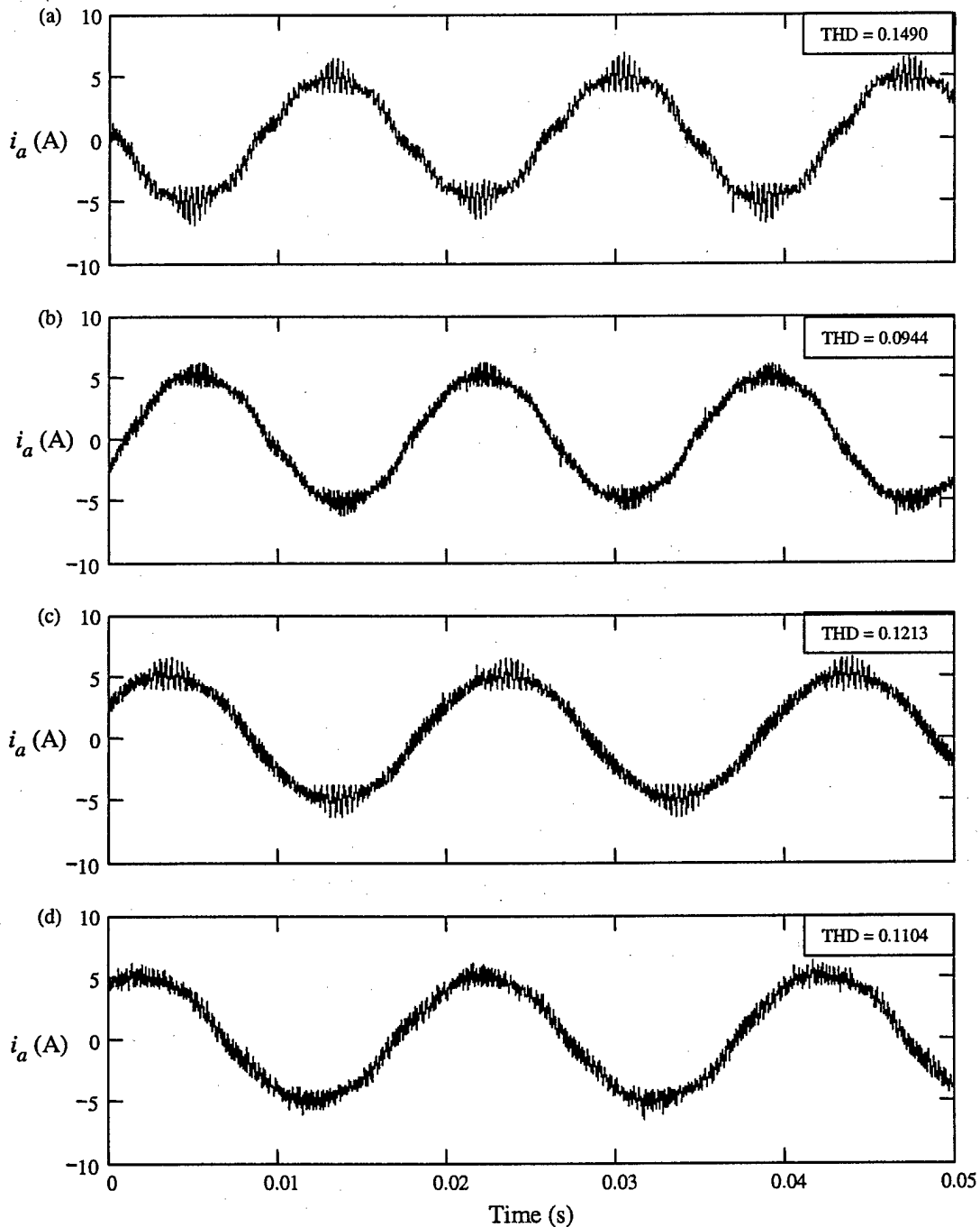
Fig. 24. Measured no-load current (a) CSVPWM at F_1=60\text{Hz} , (b) three-zone hybrid PWM I at F_1=60\text{Hz} , (c) CSVPWM at F_1=50\text{Hz} and (d) three-zone hybrid PWM I at F_1=50\text{Hz}
