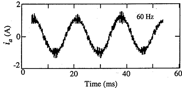
Fig. 32. No-load current waveform corresponding to five-zone hybrid PWM.
