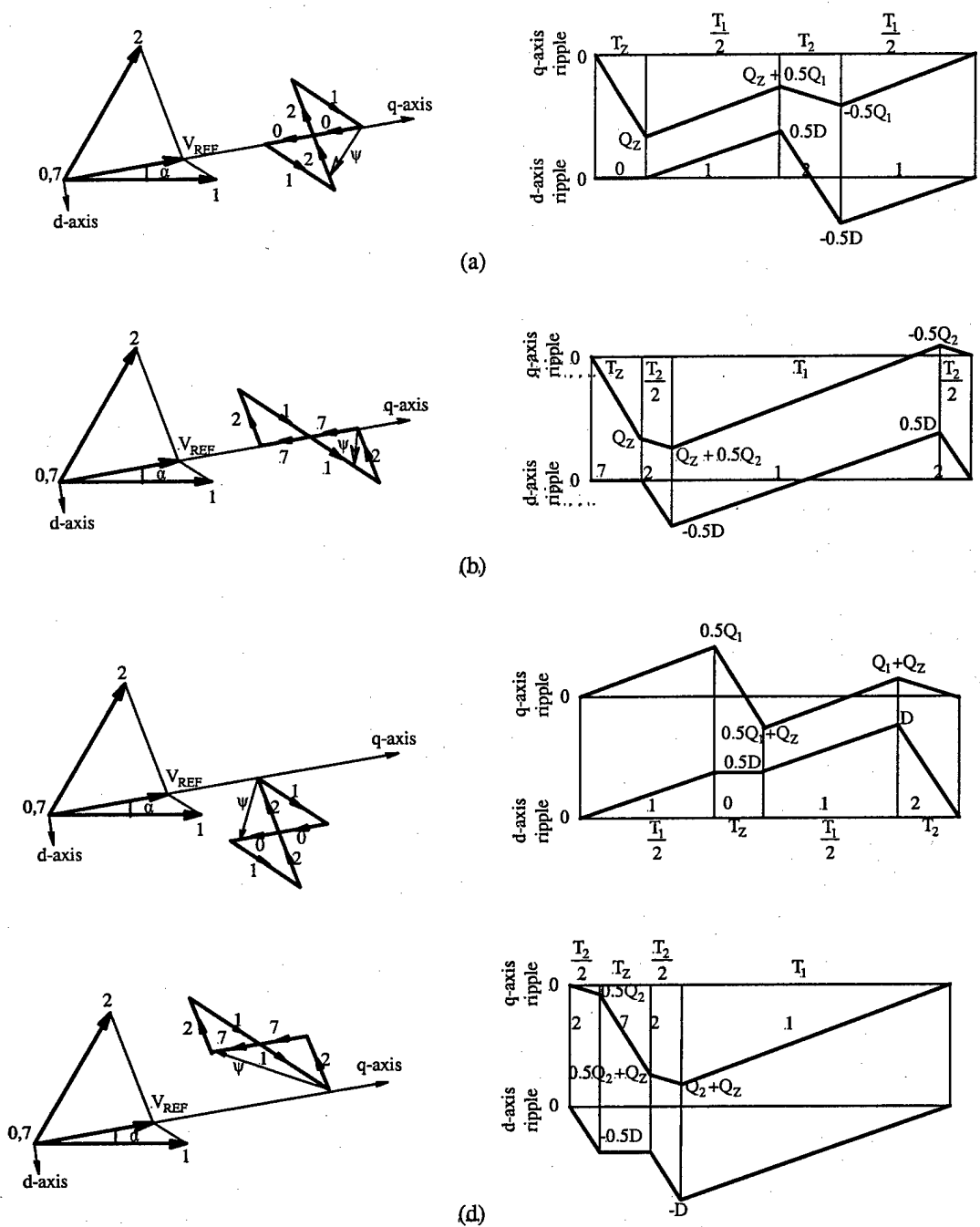
Fig. 17. Stator flux ripple corresponding to sequences (a) 0121, (b) 7212, (c) 1012 and (d) 2721
