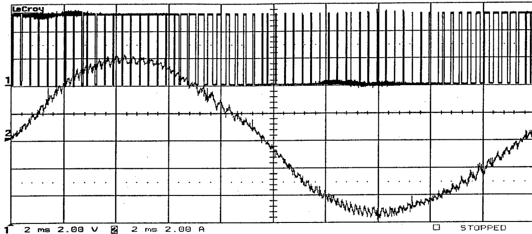
(a) Conventional SVPWM
